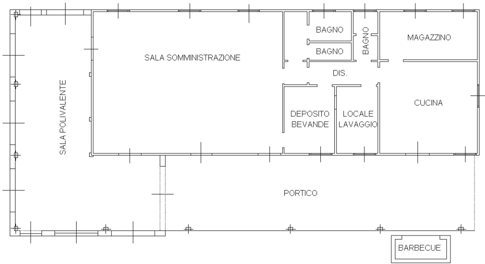
PIANO TERRA - H=270
